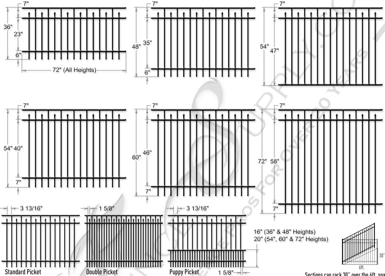
Picket Detail
