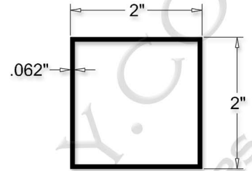
Line, Corner & End Posts Cross-Section
