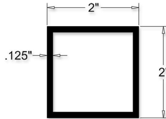
Gate Posts Cross-Section
